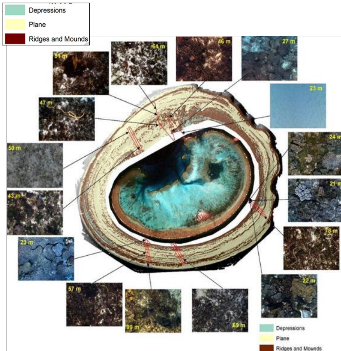
Figure 10 AUV images showing the distribution and range of benthic habitats across key geomorphological features at Middleton Reef shelf. Generally, ridges and mounds in mesophotic depths are colonised by a dense cover of hard and soft corals, with planes characterised by a mix of barren sediments and moderate cover of turfing algae, with rhodolith beds in deeper areas toward the shelf edge. AUV track lines are shown in red (From Carroll et al. 2020).
